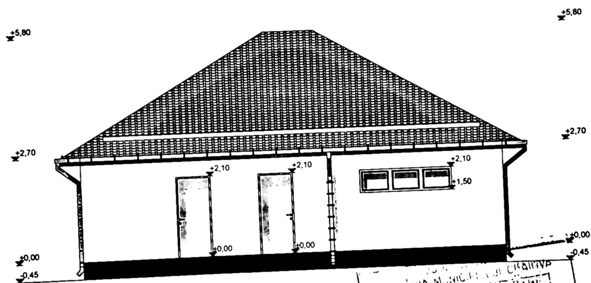
FATADA VEST
